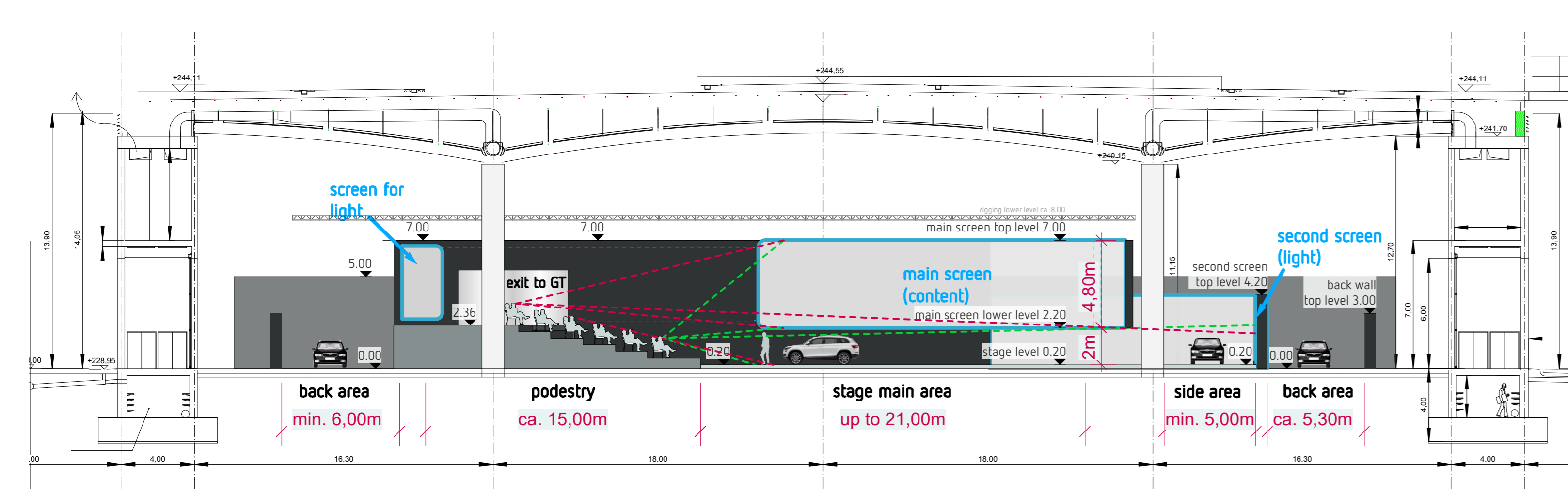
SECTION B-B
